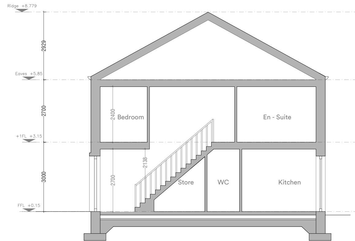
House Type P2/P3 Terraced Section A.A
