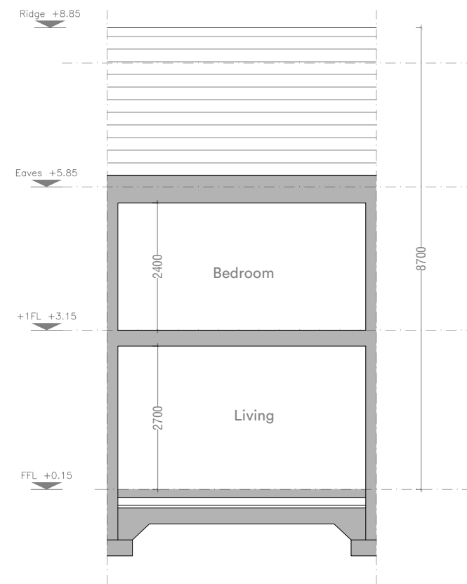
House Type P2 Terraced Section B.B
