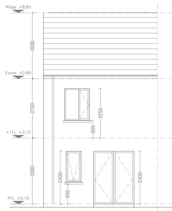
House Type P3 Terraced Rear Elevation
